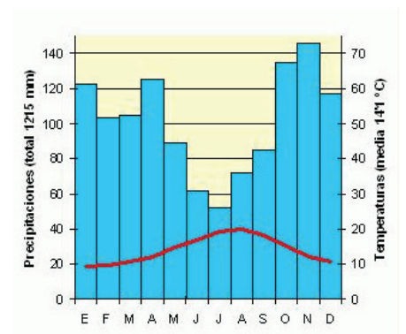
Climograma D
