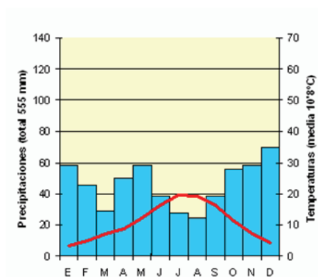
Climograma A
