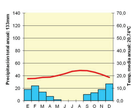
Climograma C
