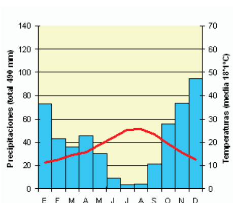
Climograma B
